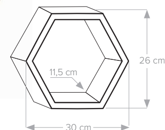
■ FHS 300 SZ index: 67702 colour: gray bulk packaging: 3 pcs
