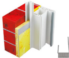
160200 L-shaped PVC reveal profile Dimension 12.5 mm
