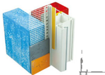
644600 Accordion PVC reveal profile with mesh for 9 mm render
