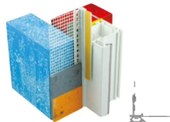
644810 Reveal profile DYNAMIK PVC with mesh / dimensions 9 mm
