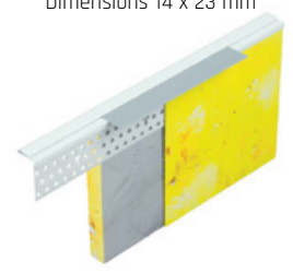
156600 PVC end profile with removable cover strips 12,5 x 30 mm
