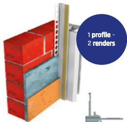
646950 PVC combi reveal profile with lip 6 and 9 mm render
